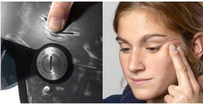
Fig. 26. Phillips Head Protection System (PHPS) (Ask Nature).
