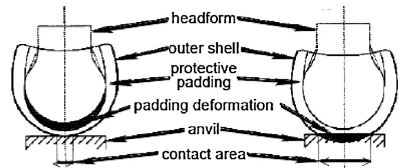
Fig. 9. Helmet deformation modes with FRP (left) and PC (right) shells (Beusenberg and Happee, 1993).
