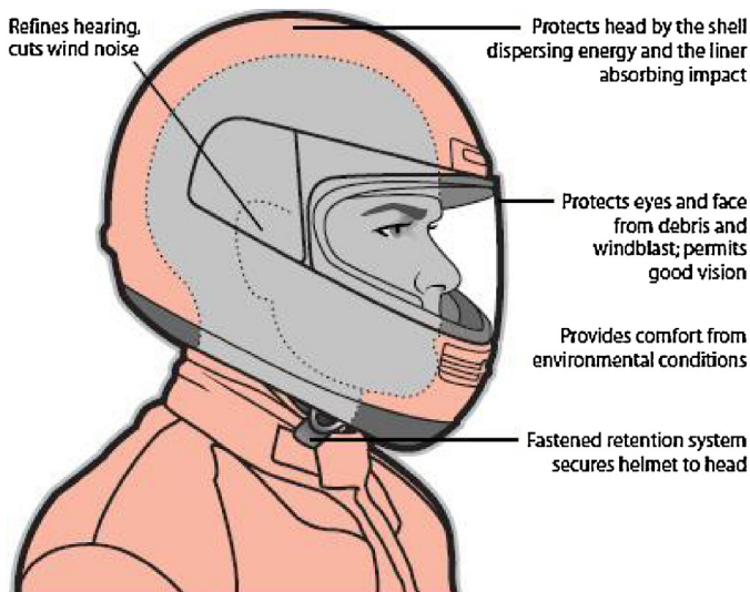
Fig. 8. Helmet components – protective/comfort functions (MSF, 2002).
