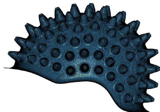
Fig. 11. ABS cone liner proposed by Blanco et al. (2010).
